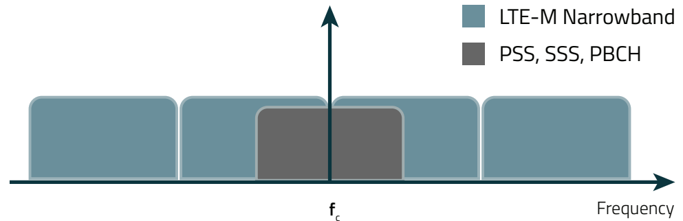
Figure 3: Arrangement of LTE-M narrowbands for a 5-MHz carrier
