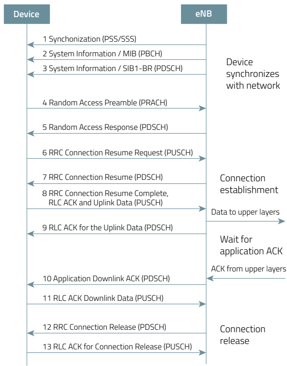
Figure 1: Message sequence for battery life and latency evaluations
