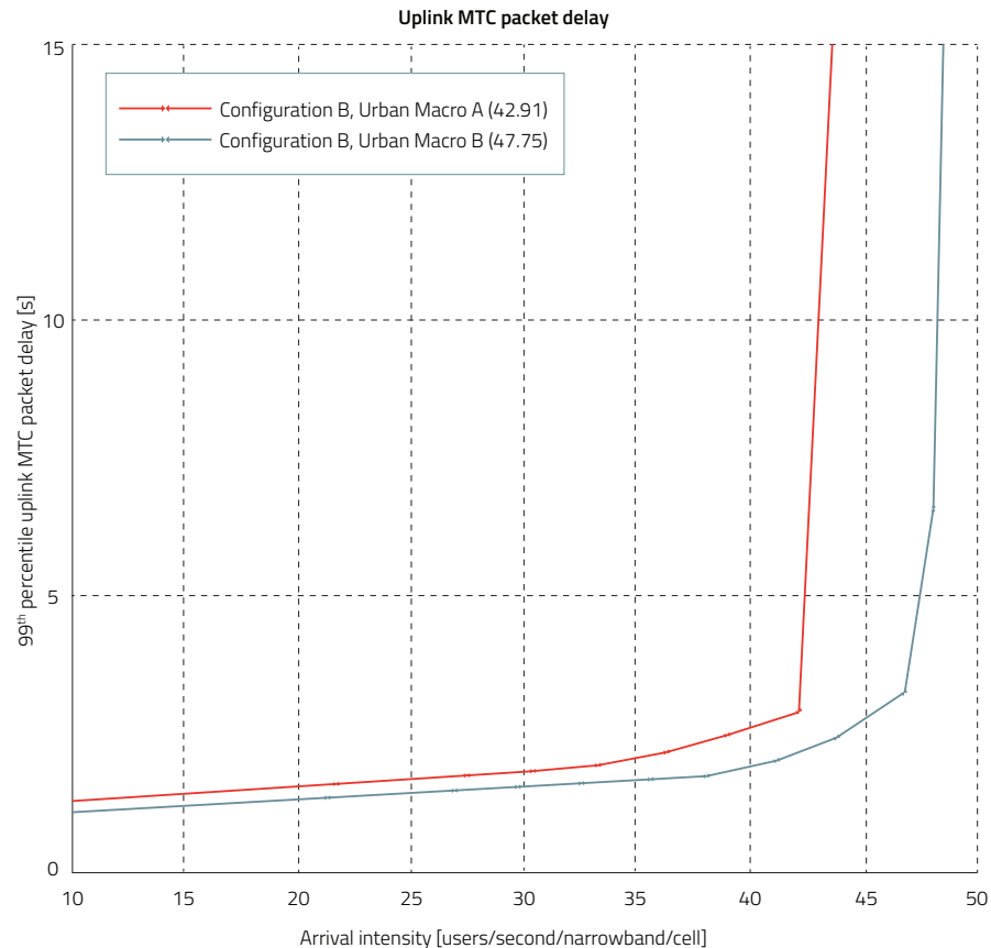
Figure 2: Service latency measured at the 99th percentile
